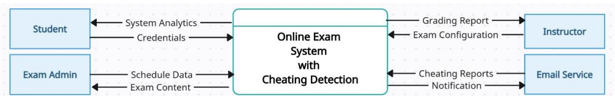
Figure 2 Context Diagram
